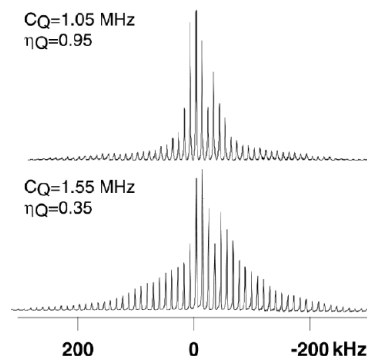
Figure 2. Example of the counterion dependence of ^{51}\text{V} MAS spectra in the Lindqvist solids [(n\text{-C}_4\text{H}_9)_4\text{N}]_3\text{H}[\text{V}_2\text{W}_4\text{O}_{19}] (top) and \text{Na}_2\text{Cs}_2[\text{V}_2\text{W}_4\text{O}_{19}]\cdot 6\text{H}_2\text{O} (bottom).
