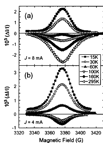
Fig. 1. The positive spin 1/2 PLDMR in Alq 3 thin films. 3
