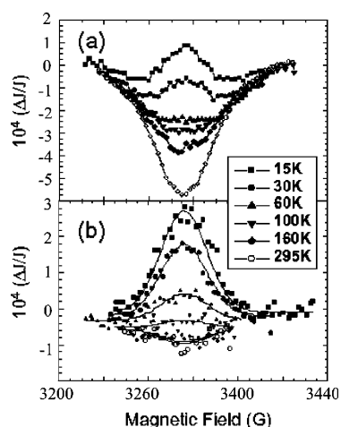
Fig. 1. The positive spin 1/2 PLDMR in Alq 3 thin films. 3
