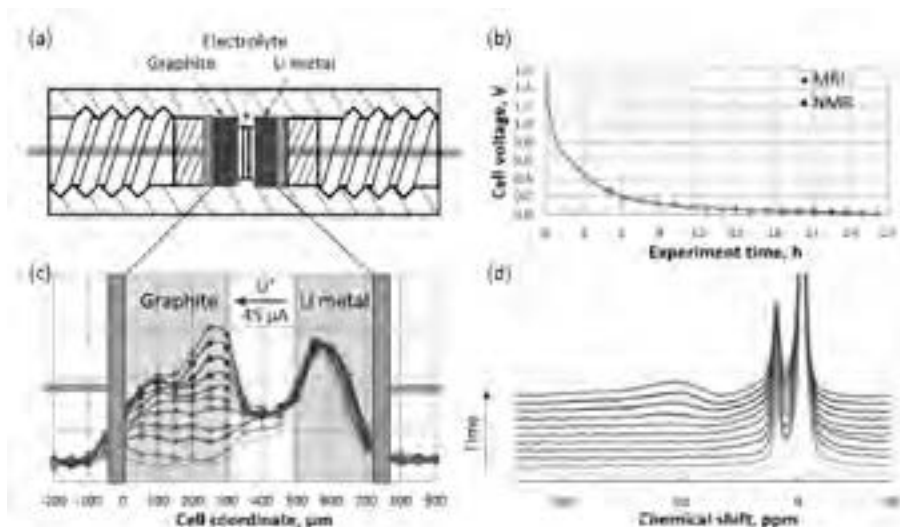
Figure 1. (a) Schematic representation of the in situ cell; (b) voltage profile of the first charging of the cell (c) axial 7 Li MR images and (d) 7 Li NMR spectra collected during the charging.
