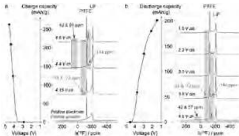
Figure 1. ^{19}\text{F} projected-MATRASS NMR spectra obtained at different stages along the full (a) charge and (b) discharge of LNF15. The points at which the electrochemical cells were stopped and the cathode material was extracted for ex situ analysis are indicated on the electrochemical curves projected on the left of the spectra. LFP-like and PTFE signals at -204 and -121 ppm, respectively, are indicated by vertical dotted lines, while F environments appearing on cycling are enclosed in yellow, blue and green rectangles.
